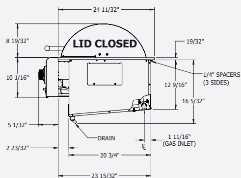
SIDE VIEW 2
