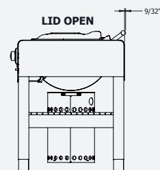
SIDE VIEW 2
