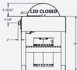
SIDE VIEW 1
