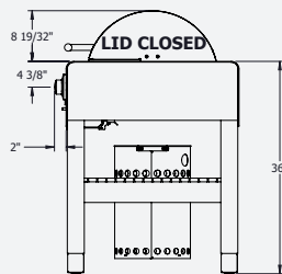
SIDE VIEW 1
