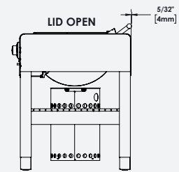
SIDE VIEW 2
