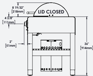
SIDE VIEW 1
