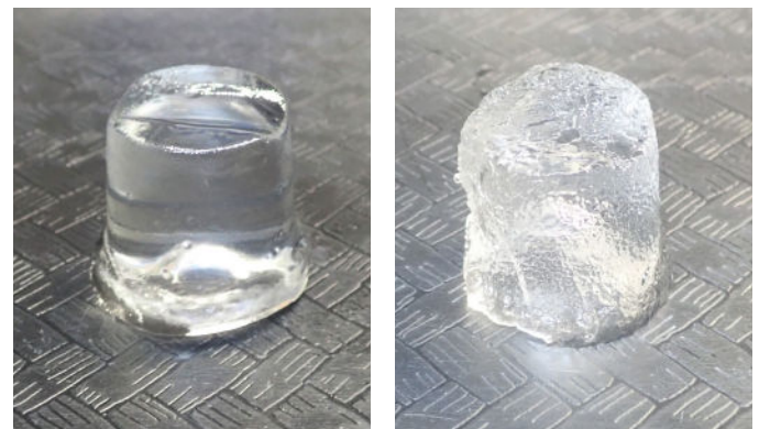
FIG. 2. Ice deteriorates and roughens as it ages.
