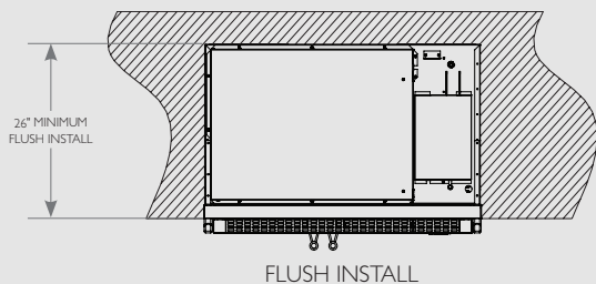
TOP VIEW FIGURE 1 - ROUGH OPENING
