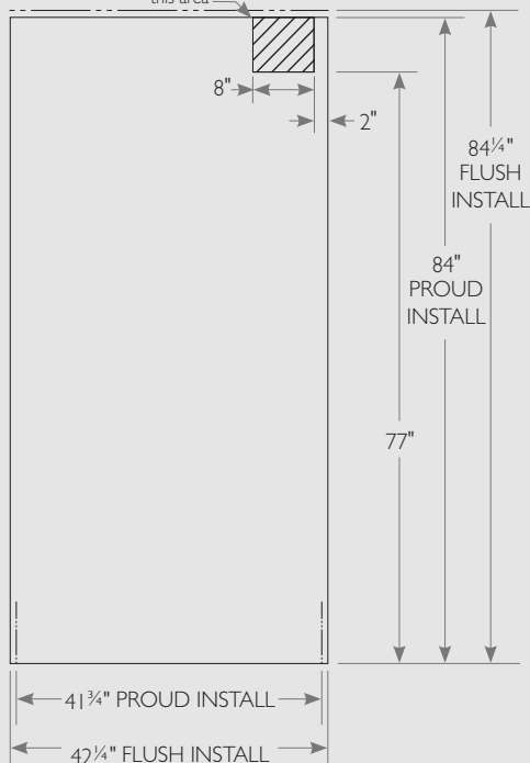
FRONT VIEW FIGURE 2 - ROUGH OPENING Electrical located in this area
